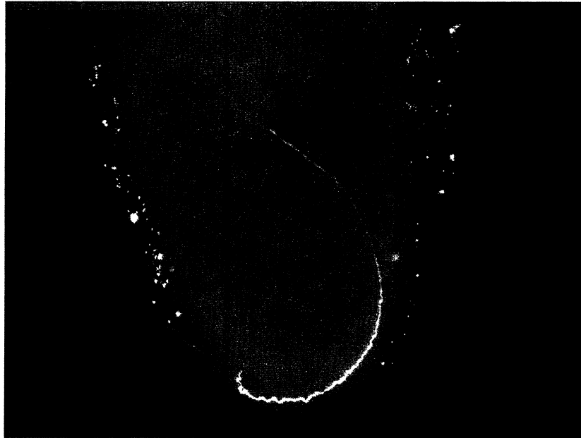
FIG. 3. Three-dimensional reconstruction of sperm in a fertilized D. pseudoobscura egg. The sperm is seen as the thin bright line extending into the egg from the anterior end (anterior is down). Carets mark 95 \mu\text{m} along the sperm, the length expected for the shorter sperm morph.
